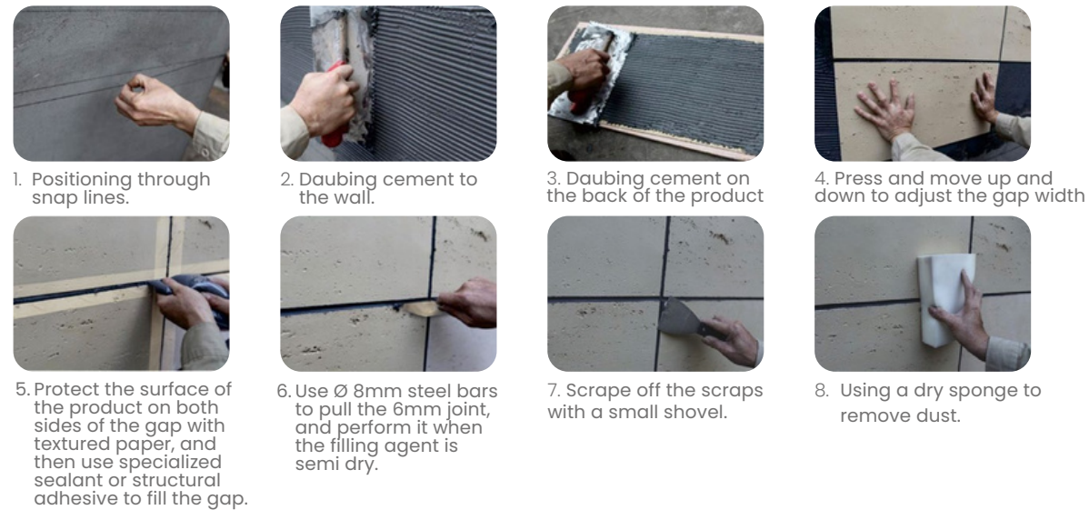
Handling process diagram
