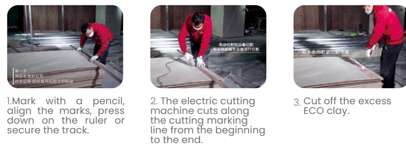
Handheld cutting machine cutting process diagram 1
